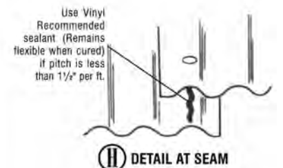
G OVERLAP DETAIL
