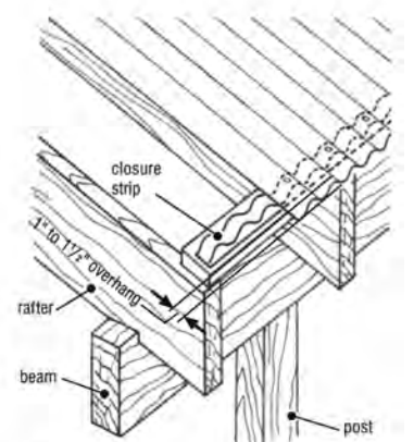
I BOTTOM CLOSURE DETAIL
