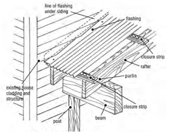
C SIDEWALL FLASHING DETAIL
