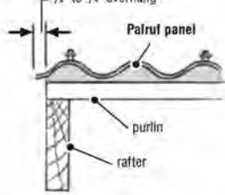
F RAKE DETAIL
