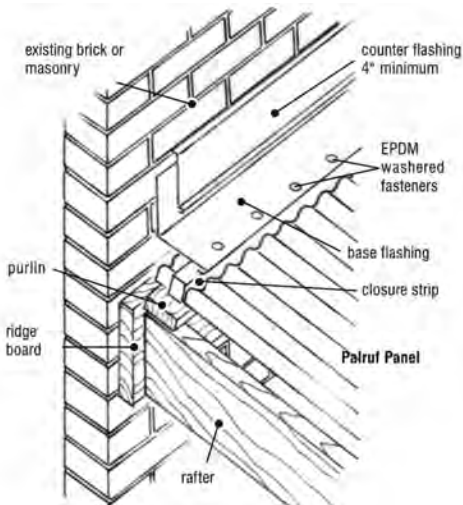
A HEAD FLASHING DETAIL AT MASONRY WALL
